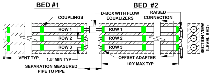
Illustration of End-to-End Multiple Beds:
