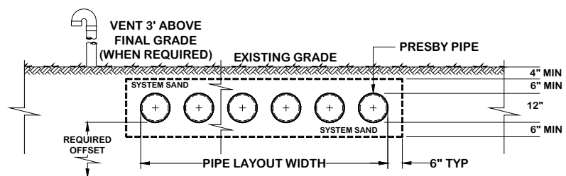
In-ground on level site:
