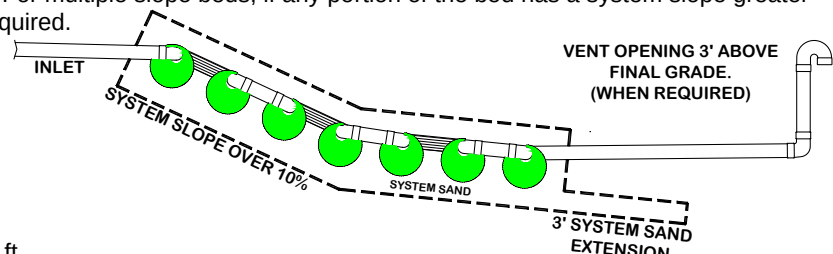
Illustration of bed with multiple slopes:
